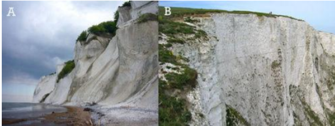
Chalk Cliffs. (A) Matching chalk cliffs in Denmark and (B) in Dover, U.K.
