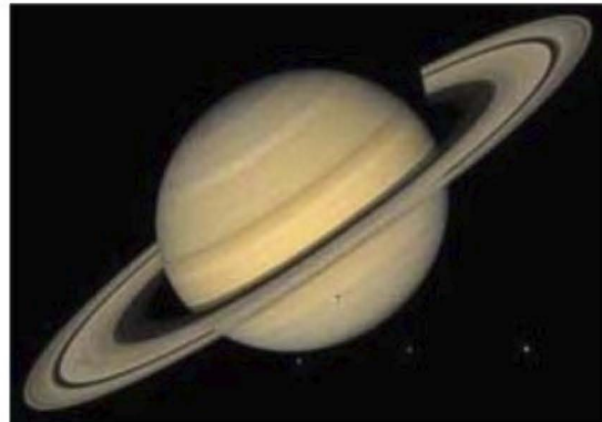
Raw digital signal sent from the Voyager spacecraft to Earth decoded by computers to show an image of Saturn, Public Domain
