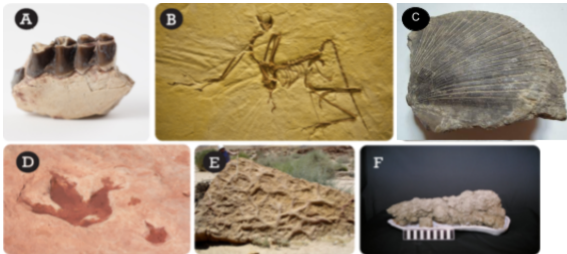
(A) furtwangl; CC-BY 2.0 (B) Hannes Grobe/AWI, CC-BY 3.0 (C) Jan Helebrant, CC-BY-SA (D) edmondo gnerre; CC-BY (E) Mark A. Wilson (Department of Geology, The College of Wooster); public domain (F) Courtesy of the U.S. Geological Survey; public domain
