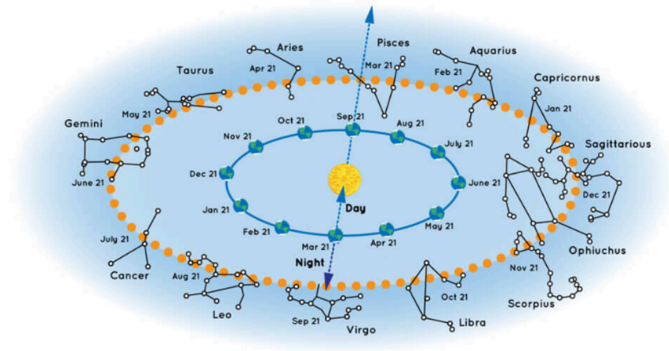
A chart showing some of the constellations that are visible from the Northern Hemisphere in different times of year. Credit: NASA/JPL-Caltech, Public Domain
