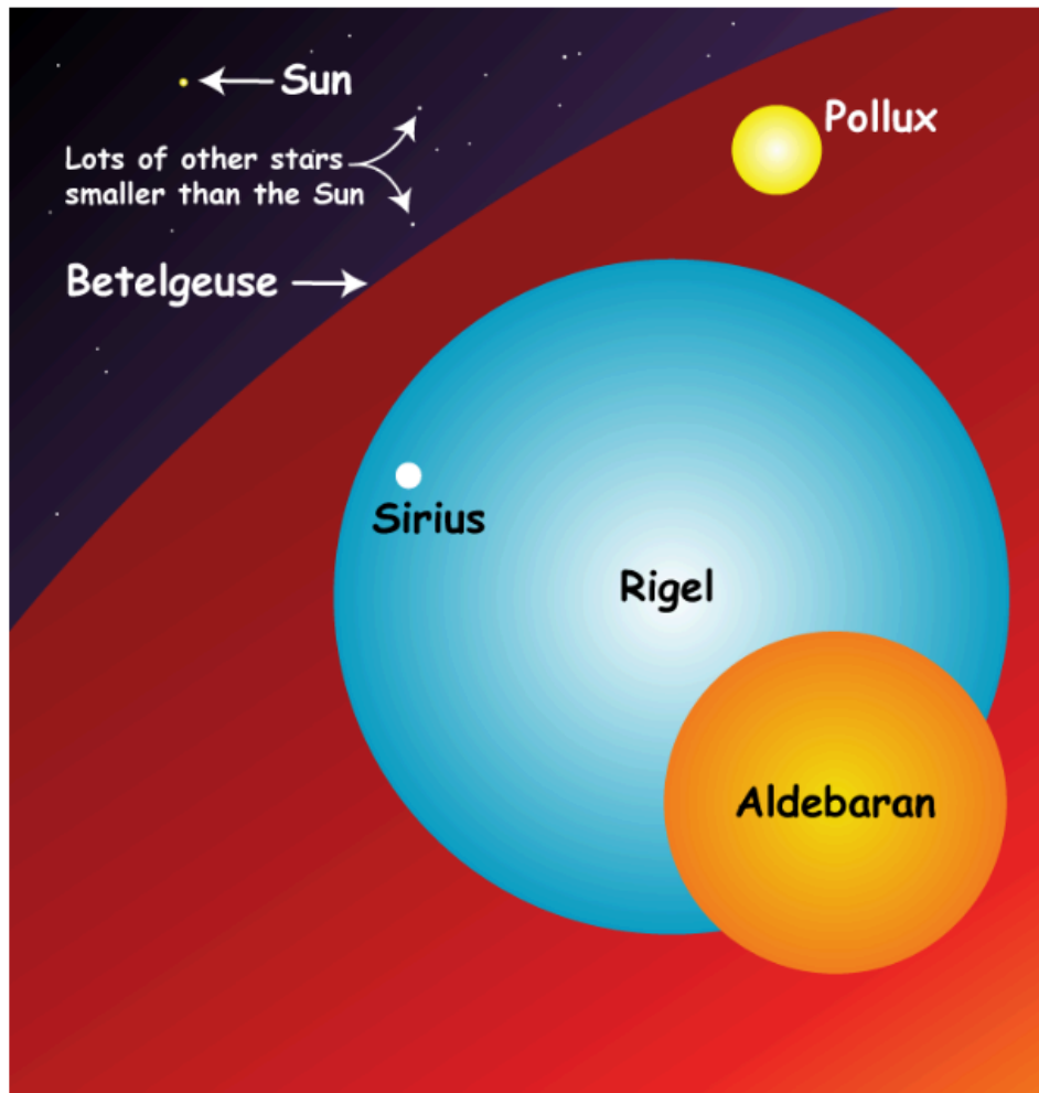
Comparison of the size of the Sun to other Stars seen in the night sky. Image by NASA, Public Domain,
