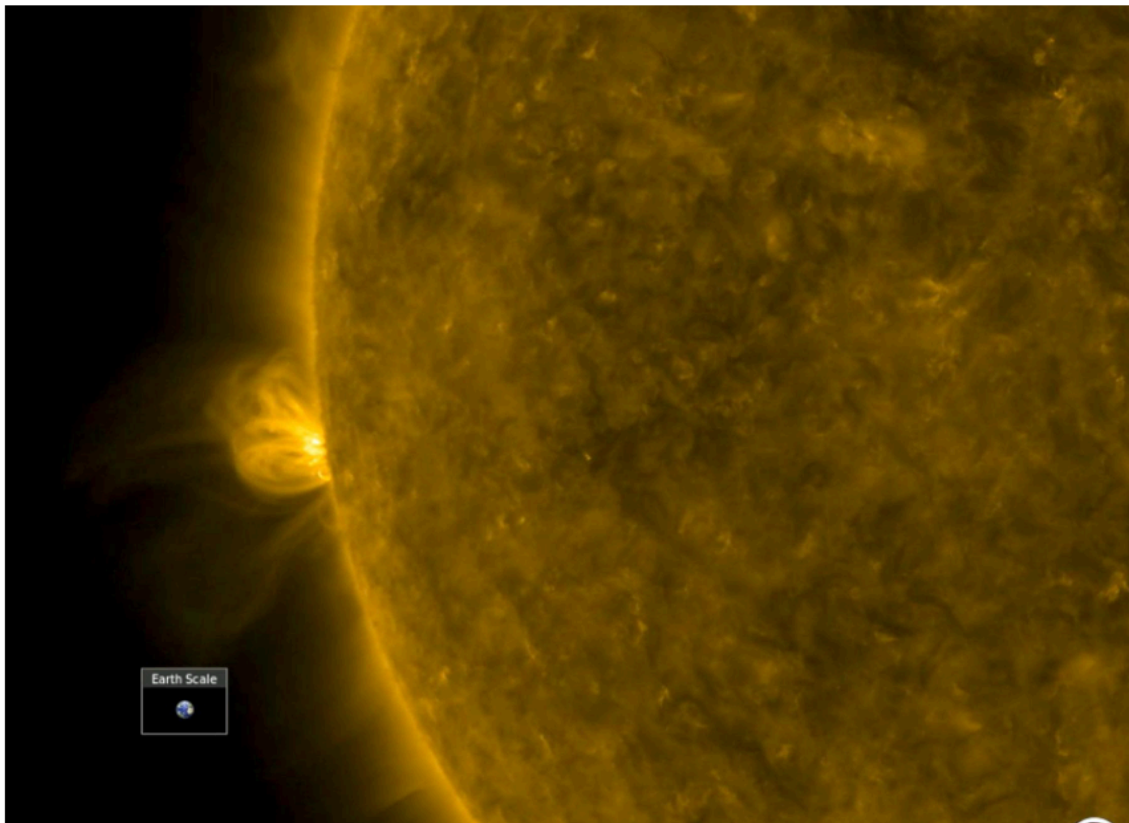
The size of the Sun and Earth shown at the same scale. Image by NASA, Public Domain
